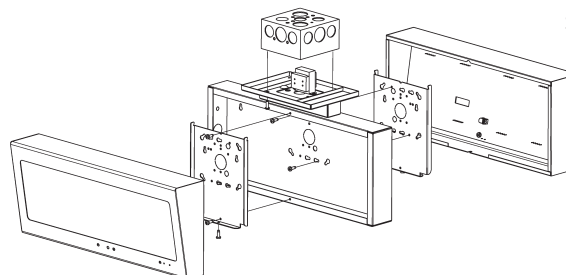
Ceiling Mounted
